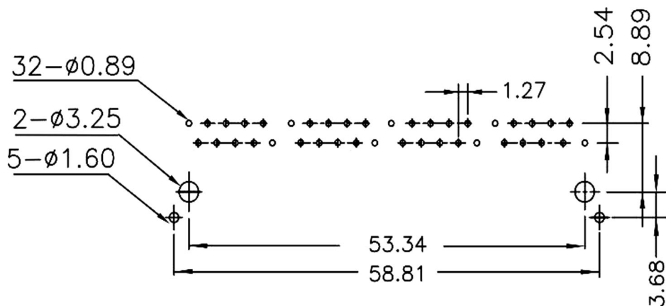
PC BOARD LAYOUT
