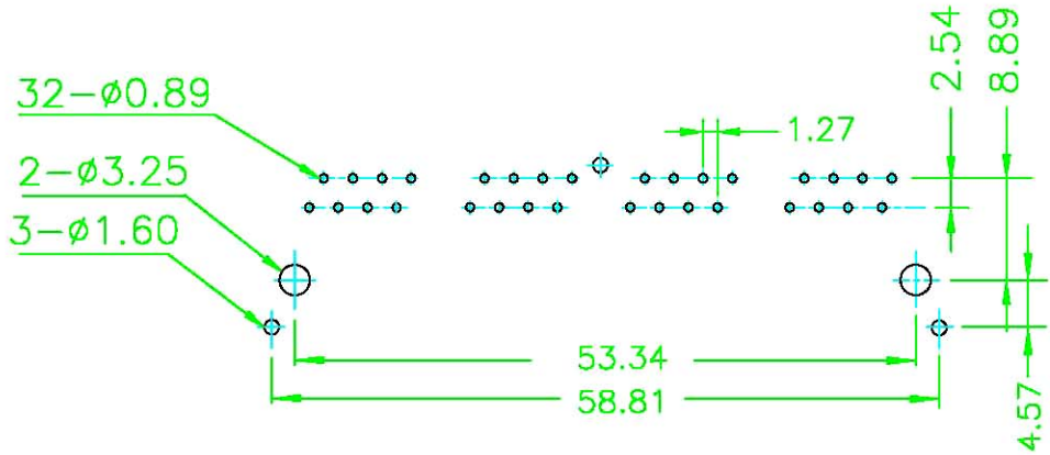
PC BOARD LAYOUT
