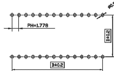
PC BOARD LAYOUT T=1.6mm
