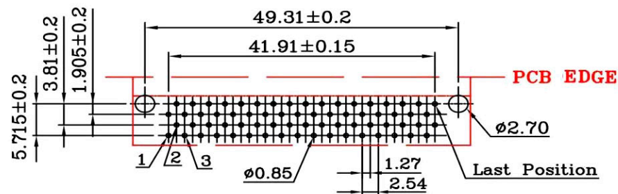
PCB Layout (REVERSE)
