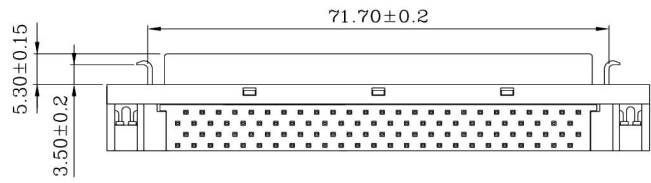
A: Metal Shell W/ Front Latch
