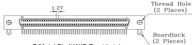
B: Metal Shell W/O Front Latch
