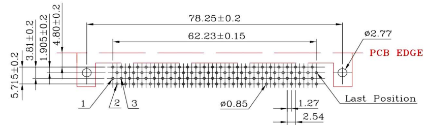
PCB Layout (B)
