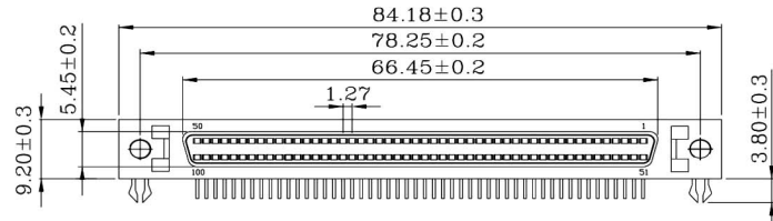
A: Metal Shell W/ Front Latch
