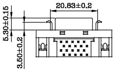
LATCH BRACKET
