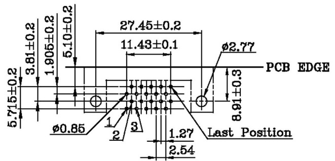
PCB Layout
