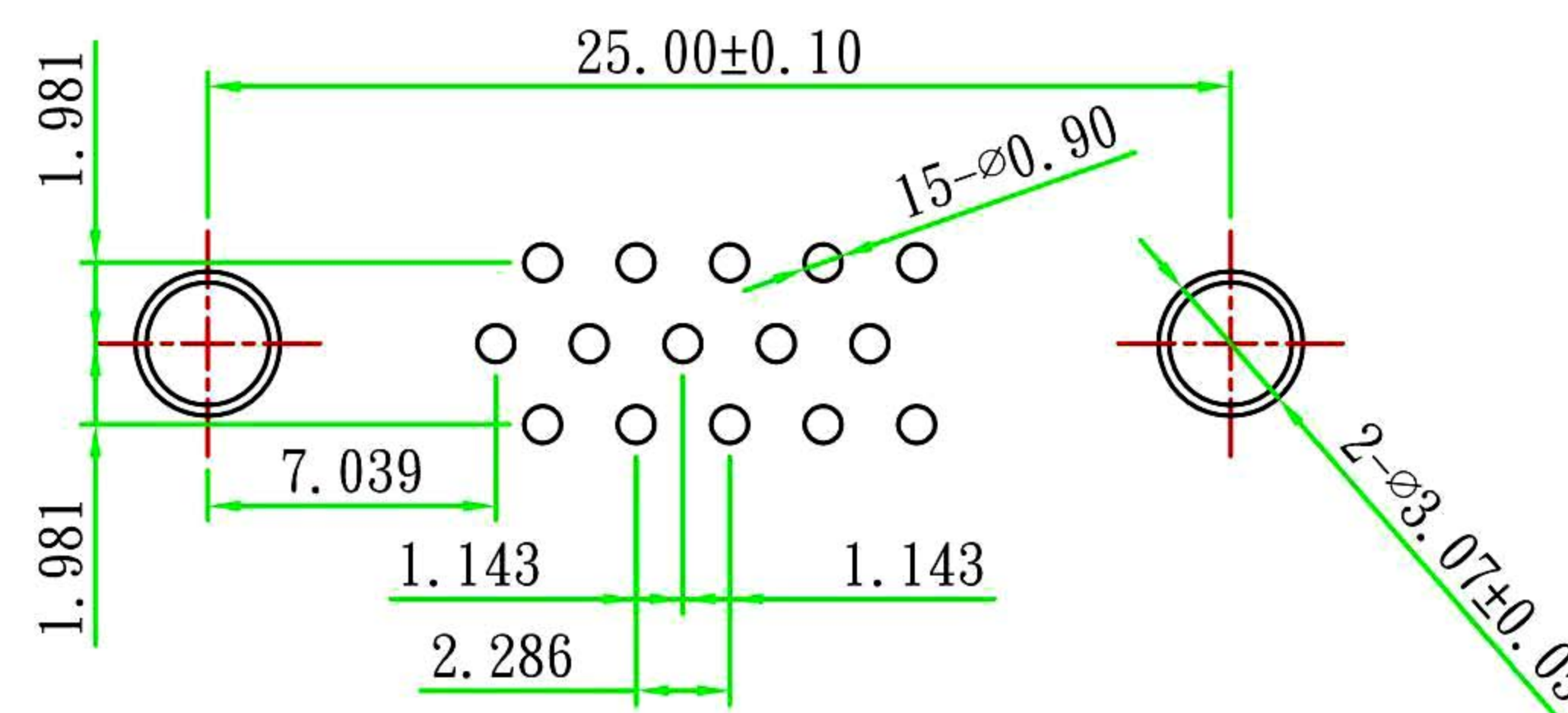
P. C. BOARD LAYOUT
