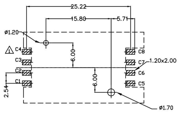
(.XX±0.05) REFERENCE PCB LAYOUT
