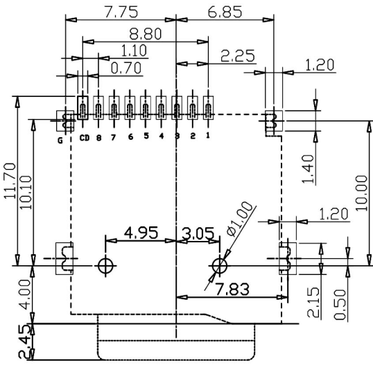
RECOMMENDED PCB LAYOUT TOLERANCE:±0.05
