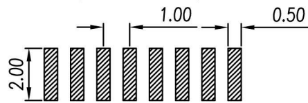
Recommended P.C.Board Layout (Tolerance: ±0.05)
