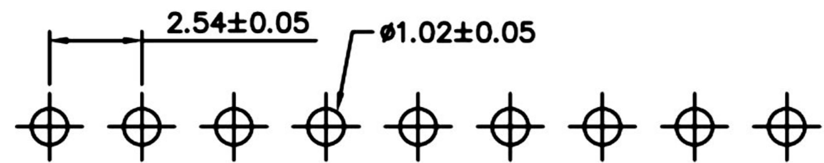
Recommended P.C.Board Hole Layout
