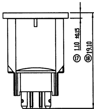
Straight Plug with Cap
