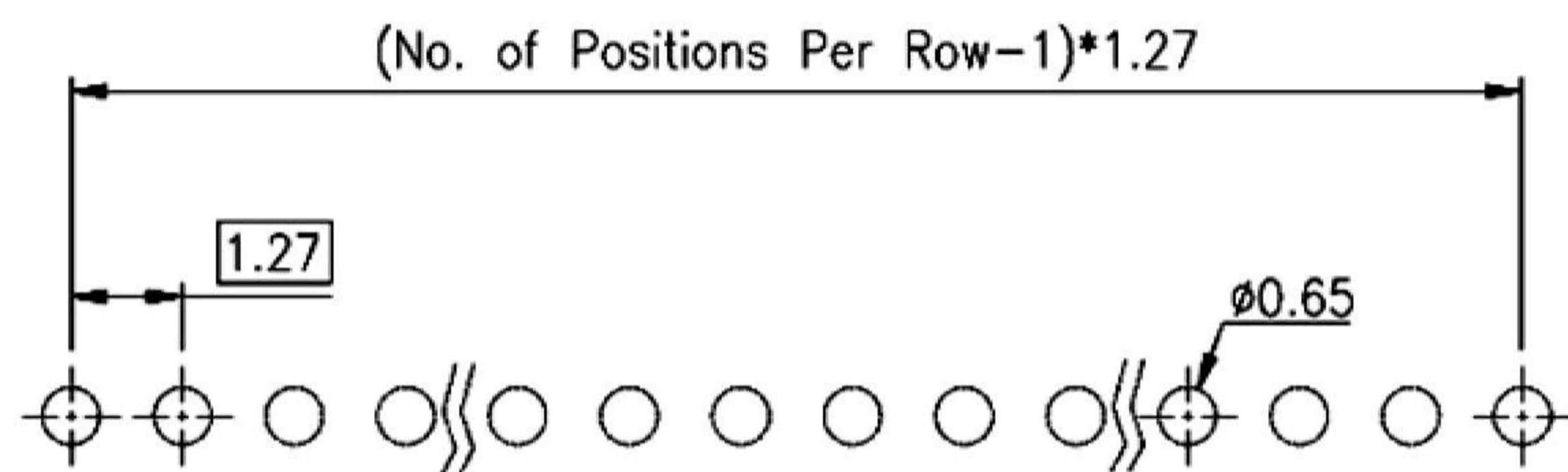
PCB Layout (Top View)
