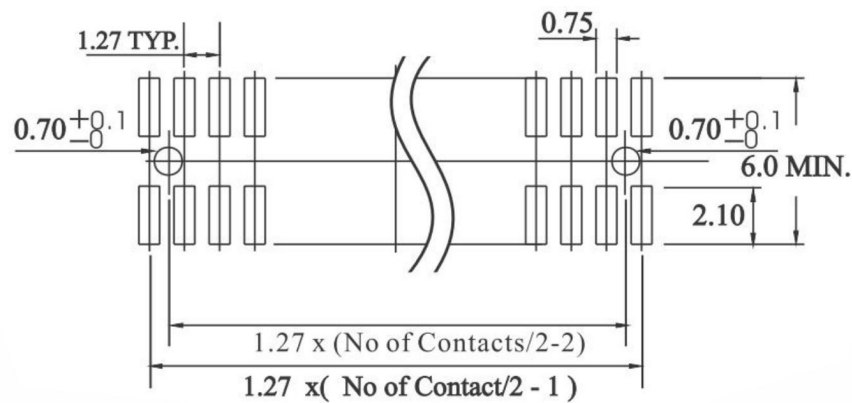
Recommended P.C.Board Hole Layout :
