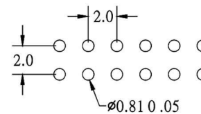
RECOMMENED P.C.B. LAYOUT
