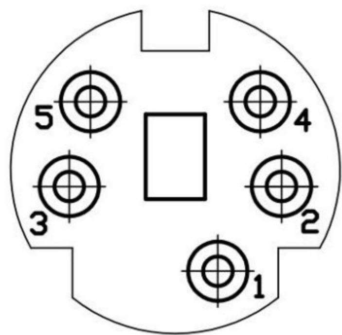
Arrangement of Contact
