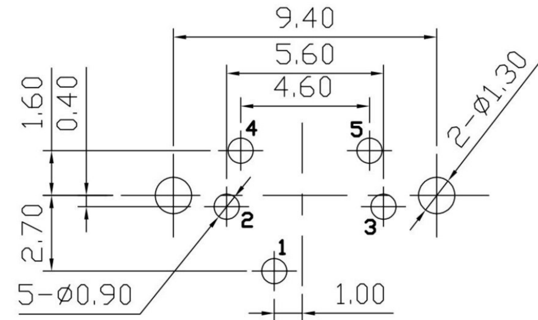
Pin Hole Layout (Jack Bottom View)
