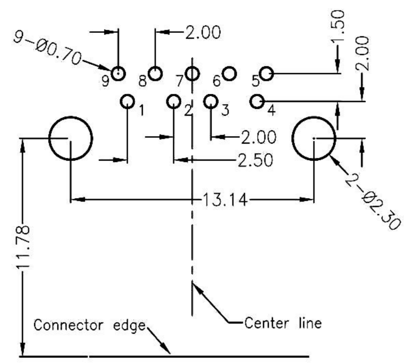
RECOMMENDED P.C.B HOLE LAYOUT (TOP VIEW) P.C.B THICKNESS=1.60mm (TOLERANCE=±0.05)
