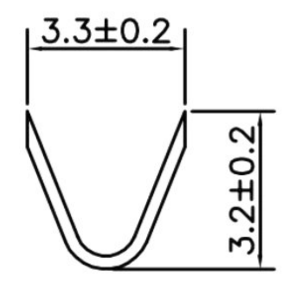
B-B Section
