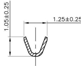
A-A SECTION ( INSULATION BARREL )
