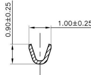
B-B SECTION ( WIRE BARREL )
