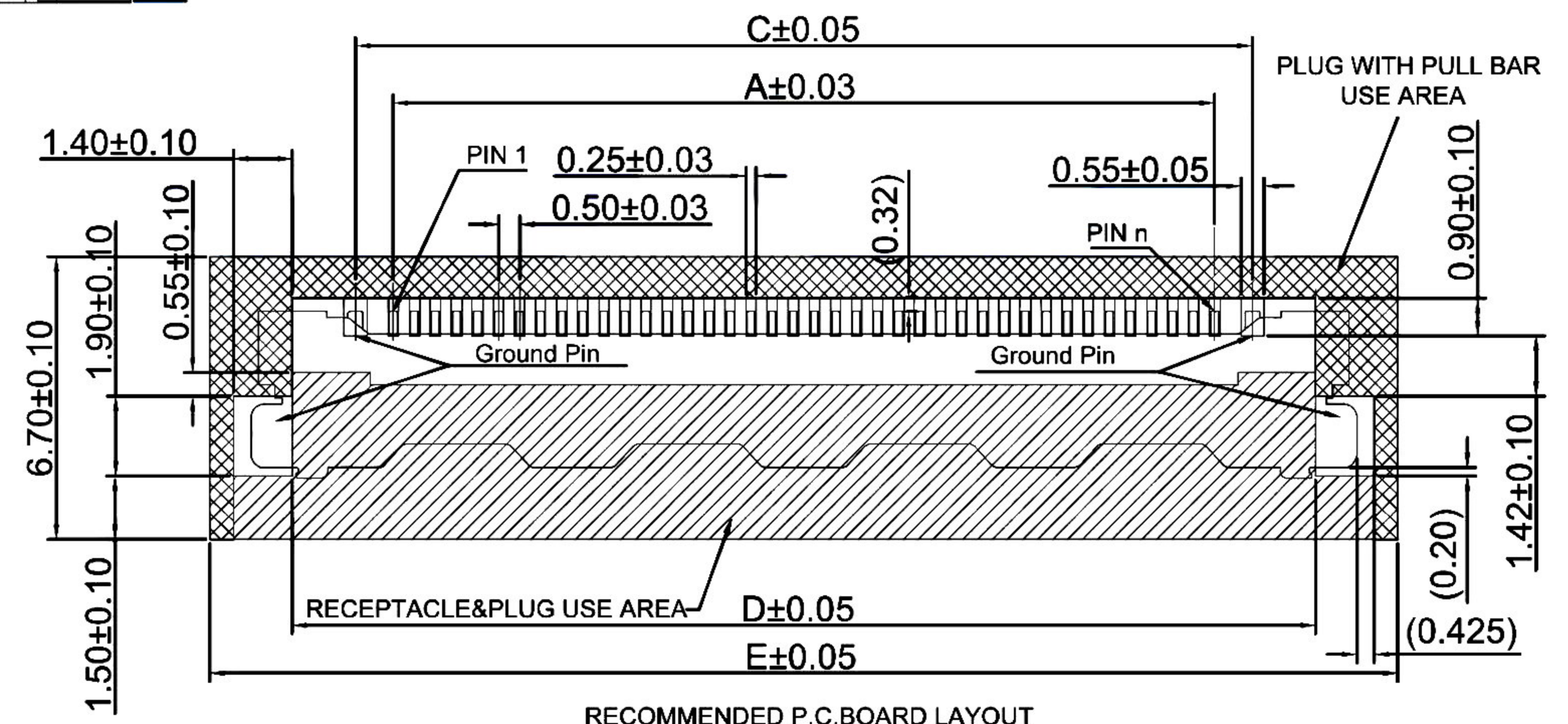
RECOMMENDED P.C.BOARD LAYOUT
