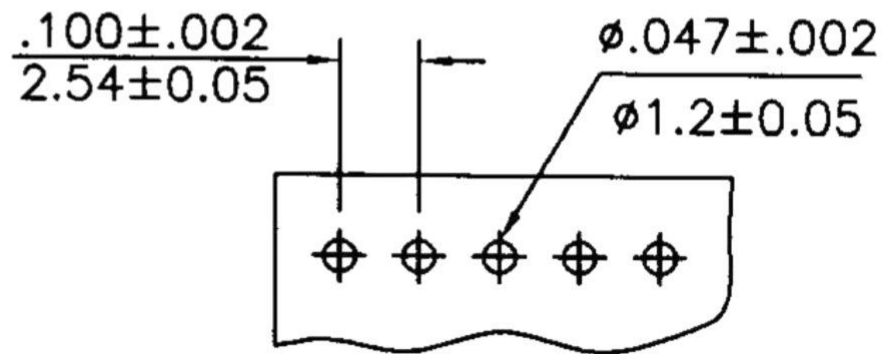
P.C. Board Layout
